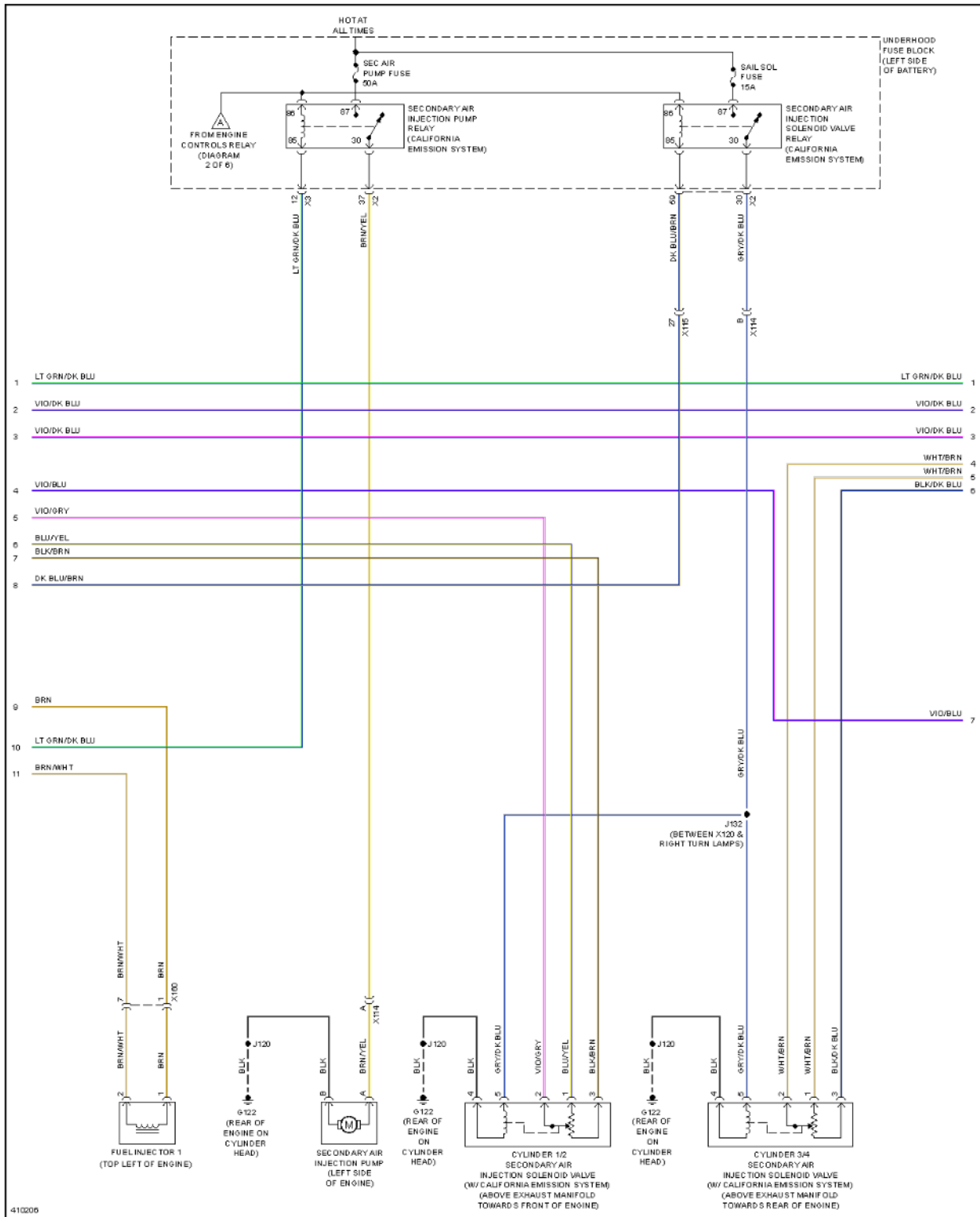
Fig. 39: 2.4L VIN R, Engine Controls Circuit (5 of 6)
