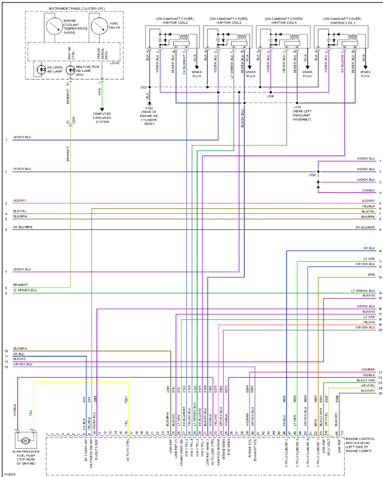
Fig. 37: 2.4L VIN R, Engine Controls Circuit (3 of 6)
